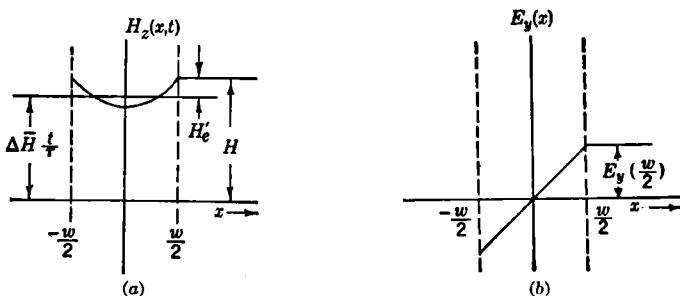
FIG. 15-25.—Steady-state distribution throughout the core of (a) H_z(x,t) , where H_c' = \frac{10^{-9}\mu\pi w^2\Delta H}{3r\left(\frac{r_0}{d}\right)} oersteds, and (b) E_y(x) , where E_y\left(\frac{w}{2}\right) = \frac{10^{-6}\mu\Delta H w}{2r} volts.
